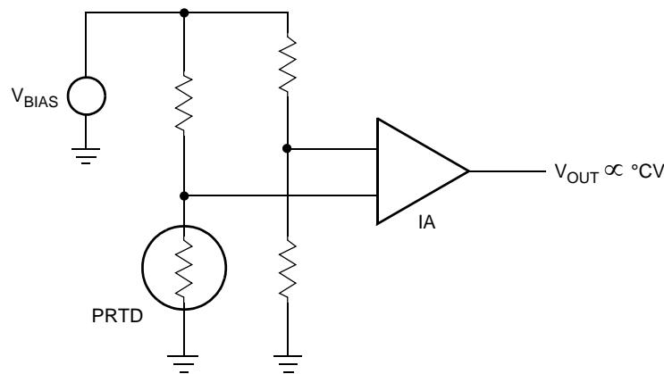
FIGURE 5. PRTD SENSOR CIRCUIT – BASIC
