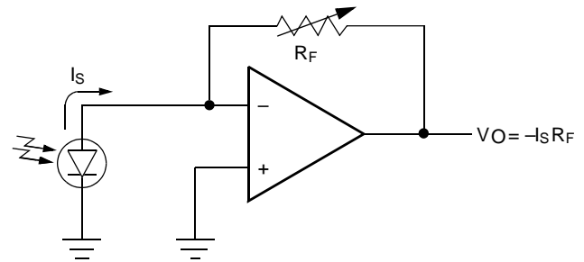
FIGURE 1. TRANSIMPEDANCE AMPLIFIER
