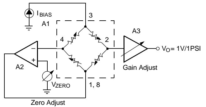
FIGURE 3. PRESSURE TRANSDUCER SIGNAL CONDITIONING CIRCUIT – SIMPLIFIED
